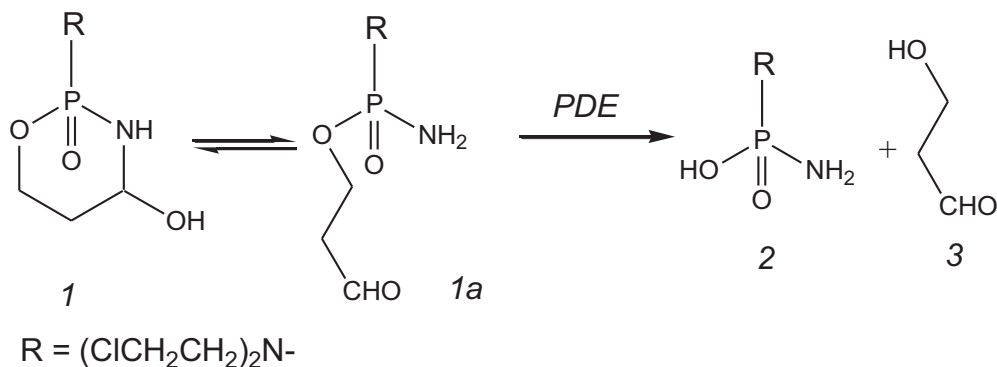
Fig. (6). Reaction scheme for enzymatic decomposition of OHCP/ALDO by phosphodiesterases (PDE), 1 OHCP, 1a ALDO, 2 PAM, 3 3-hydroxypropionaldehyd.
