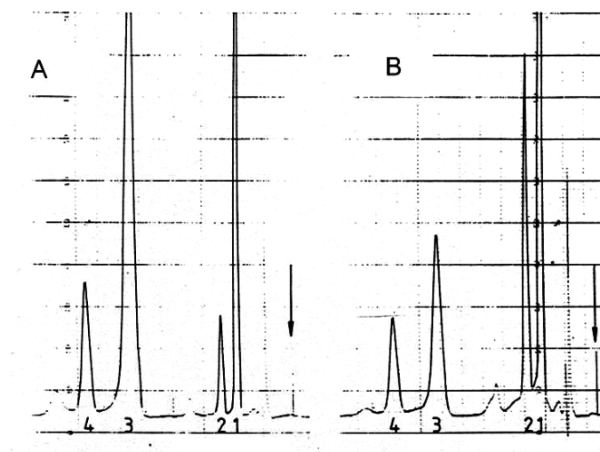
Fig. (5). HPLC analysis of aliquots of OHCP incubated in rat serum (pH7, 37°C) for 10 min (A) or 90 min (B). Proteinprecipitation and reaction of the aldehydes with 2,4 dinitrophenylhydrazine. 1: 2,4 dinitrophenylhydrazine, 2,3,4: dinitrophenylhydrazones of hydroxypropanal (2), aldophosphamide (3) and acrolein (4). Arrows indicate start of HPLC run.
