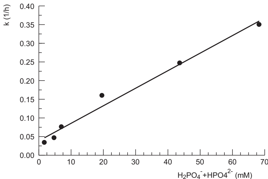
Fig. (1). Formation of PAM from OHCP/ALDO as a function of concentration of \text{H}_2\text{PO}_4^- + \text{HPO}_4^{2-} , in protein free rat serum ultrafiltrate pH7, 37°C. k (1/h) is the first order rate constant of the formation of PAM form 4-OHCP.
