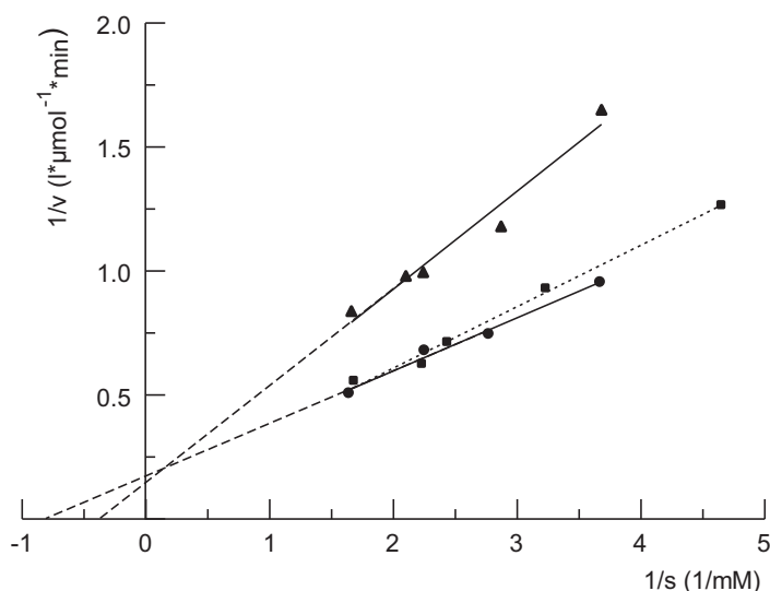
Fig. (4). Lineweaver-Burk plot for enzymatic decomposition of OHCP/ALDO by snake venom phosphodiesterase (EC 3.1.4.1.) (●) and effect of 5' AMP (▲) and 3' AMP (■) on decomposition activity. Photometric determination of NADPH+H + after addition of snake venom phosphodiesterase to a solution containing NADP, aldehyde dehydrogenase and OHCP in phosphate buffer.
