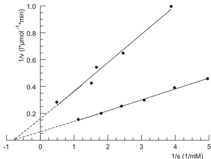
Fig. (3). Lineweaver-Burk plot for decomposition of OHCP/ALDO by human serum. Start of reaction by adding 50 \mu l or 100 \mu l (lower line) human serum. Photometric determination of NADPH+H + after addition of human serum to a solution containing NADP, aldehyde dehydrogenase and OHCP in phosphate buffer.
